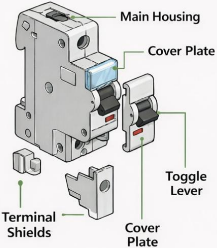
Miniature Circuit Breaker (MCB)
