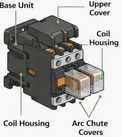
Contactor
